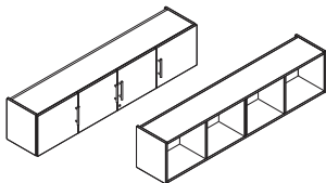
Wall Mounted Overheads With or Without Hinged Doors 16 High, 36 - 72 Wide
