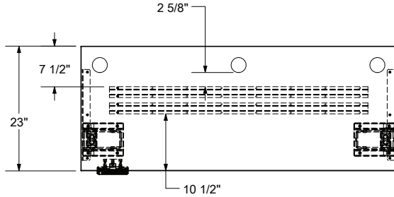
Grommet Location for 30" Deep Single Tables
