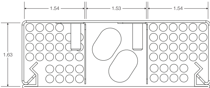
Power pole with feed with center barriers = 64 CAT 6 cables
