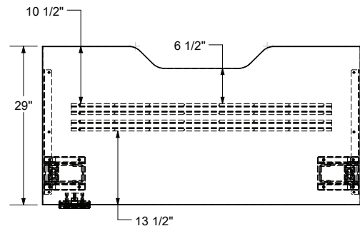
Scallop Location for 30" Deep Single Tables
