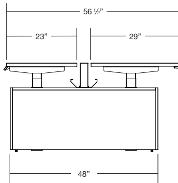
Encounter PowerBench 48D Laminate Base (1) 30D Encounter PowerBench HATs for Double Bench (1) 24D Encounter PowerBench HATs for Double Bench
