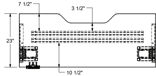
Scallop Location for 24" Deep Single Tables
