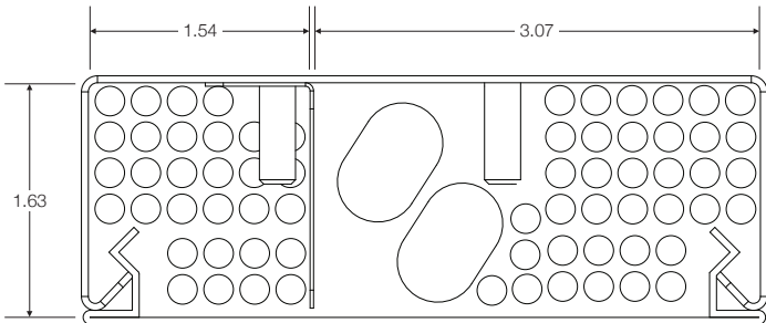
Power pole with feed with one center barrier = 66 CAT 6 cables
