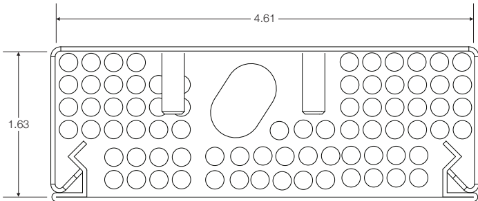
Power pole with feed with no center barriers = 88 CAT 6 cables
