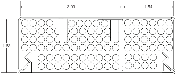
Power pole with no feed = 97 CAT 6 cables
