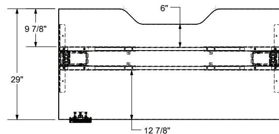
Grommet Location for 30" Deep Double Tables
