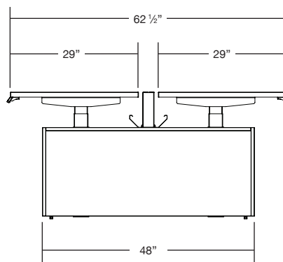
Encounter PowerBench 48D Laminate Base (2) 30D Encounter PowerBench HATs for Double Bench
